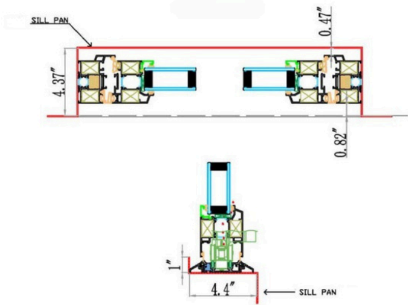
Sill Pan Details
